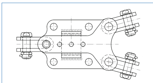
Groundwire bracket
